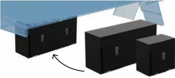
Underbody Box L450 x W300 x H450 mm L600 x W300 x H450mm L750 x W300 x H450mm L900 x W300 x H450 L1200 x W300 x H450 Truck underbody aluminum box, available in a range of sizes, are lockable and offer an additional secure storage space, making good use of under body space.
