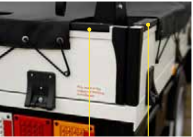
Dropside Protective Covering Black poly edging. Protection from paint chipping and dents for a more professional look in front of clients. Boosts resale value and helps items slide over the dropside edges.
