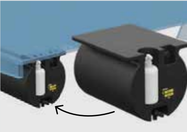
Underbody Poly Water Tank, 60L, Soap Dispenser 60L underbody water tank with soap dispenser.
